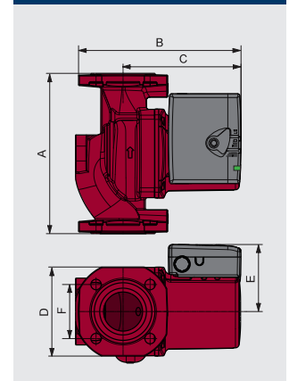
UPS 50-60
